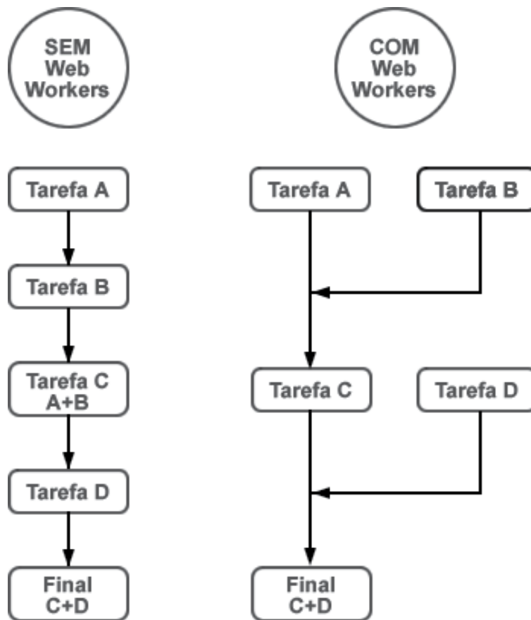
Figura 9.3 – Diagrama comparativo JavaScript x Web Workers.
