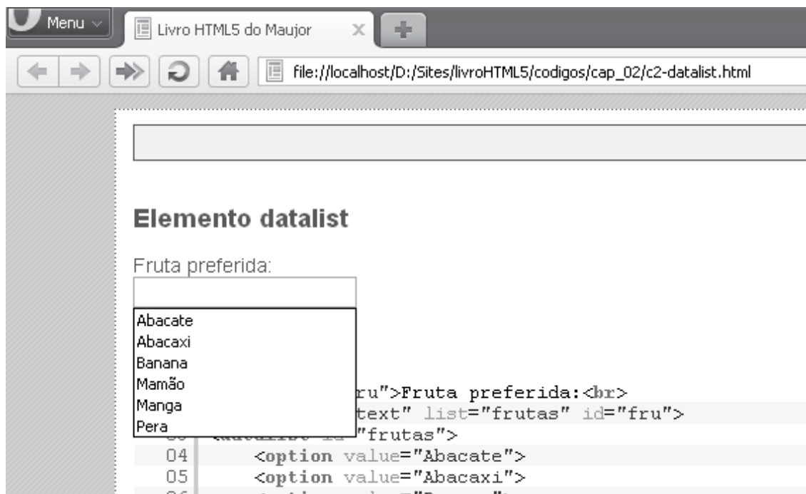
Figura 2.3 – Elemento datalist.
