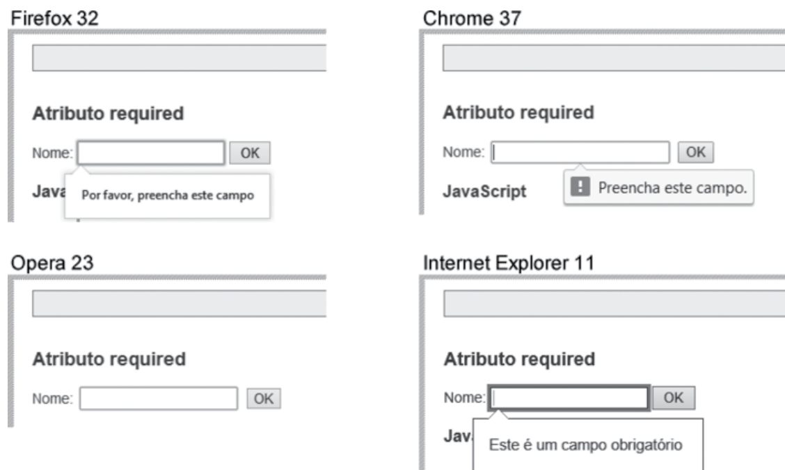
Figura 6.1 – Atributo required.
